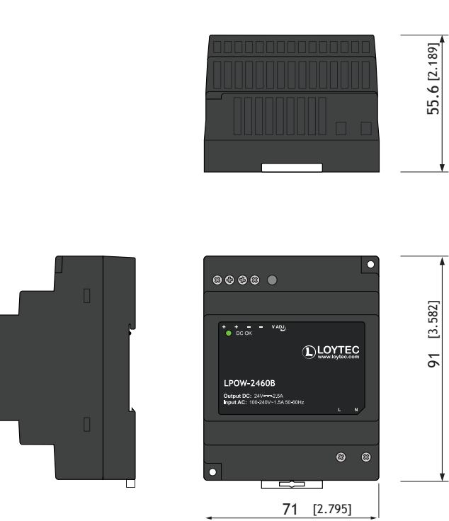
DIM050 LPOW-2460B
