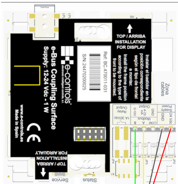
e-Bus Coupling Surface RS-485
